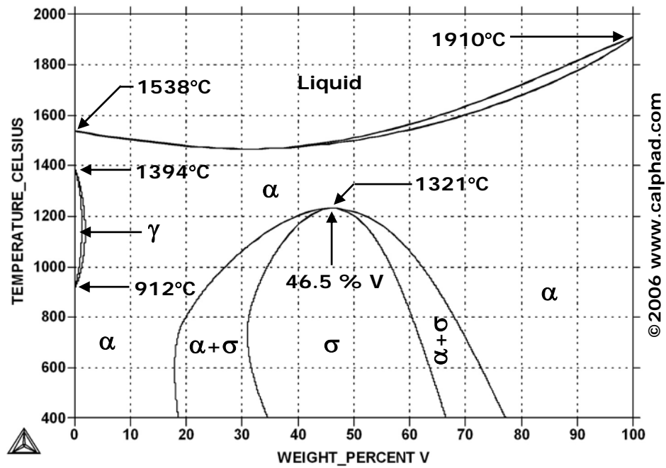
Iron-Vanadium Phase Diagram
